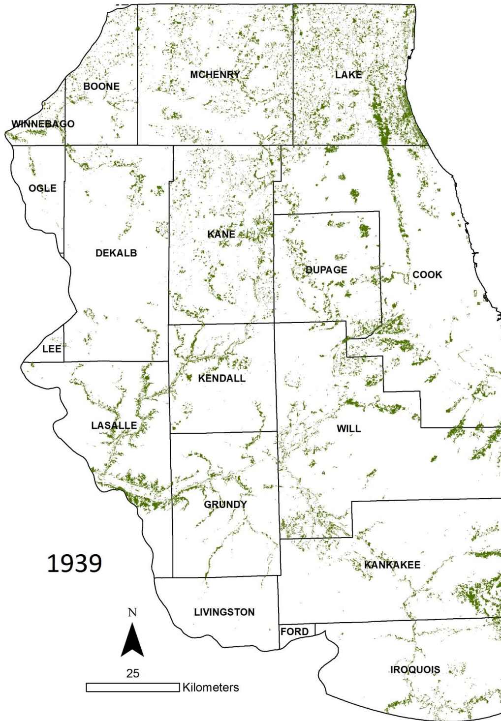
Distribution of remnant oak ecosystems based on 1939 aerial image analysis in 1939.
