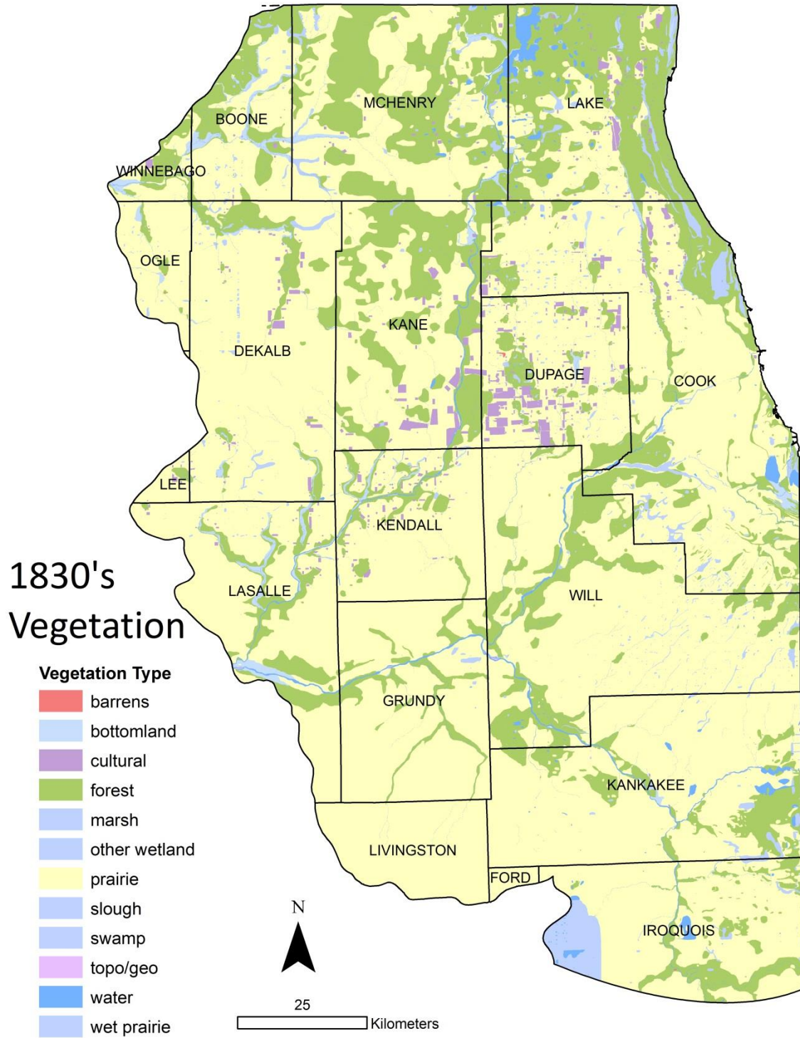
Landscape condition at the time of initial Euro-American settlement in the 1830's
