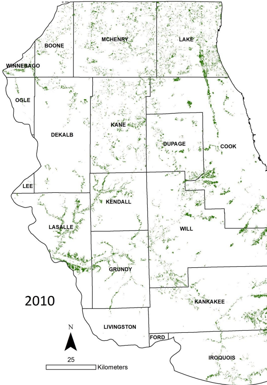
Distribution of remnant oak ecosystems based on aerial image analysis in 2010.
